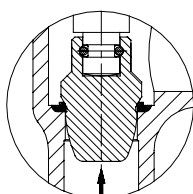
Throttle plug "RR"
