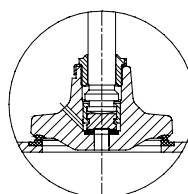
Equilibrating disc DN 125-300
