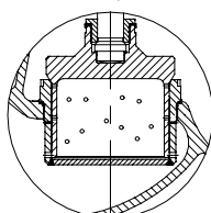
Throttle plug "Q"
